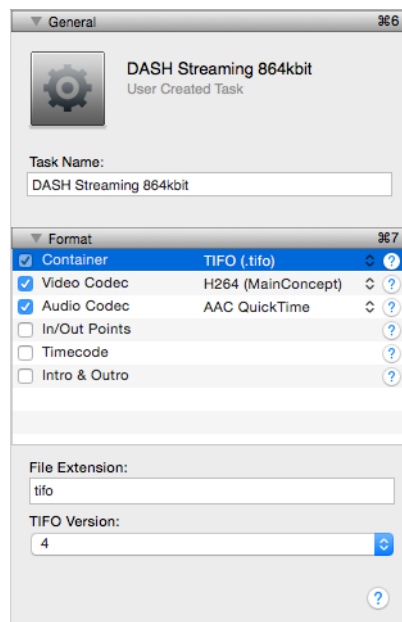
Figure 75. DASH Encoder Example
