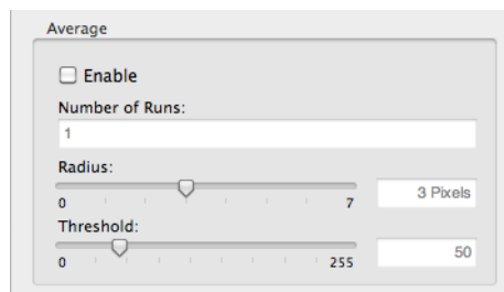
Figure 193. Noise Reduction Filter Settings—Average Method
