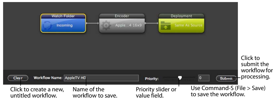
Figure 30. Workflow Editor with Typical Workflow
