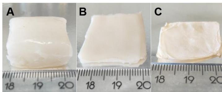
Figure S2.1 Optical images of wet BC hydrogel (A) before (thickness is 10 mm) and (B) after squeezing, and (C) after air-dried BC. BC loses over 99 % of its weight after drying in air and becomes a 2D film.
