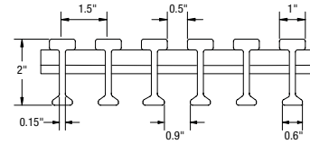
2" DEEP, T-3320 ADA COMPLIANT
