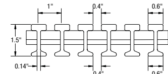
1-1/2" DEEP, I-4015 ADA COMPLIANT
