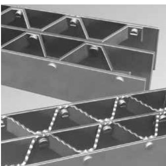
Bridge Decking
