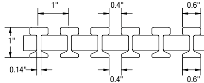
1" DEEP, I-4010 ADA COMPLIANT
