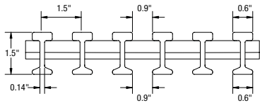
1-1/2" DEEP, I-6015
