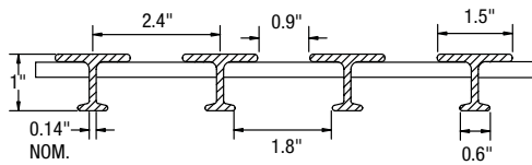
1" DEEP, T-3810
