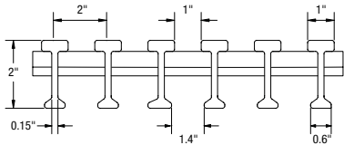
2" DEEP, T-5020
