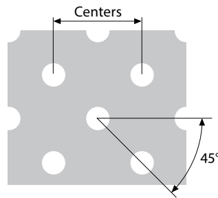
OPTIONAL ROUND PERFORATIONS 45° STAGGERED
