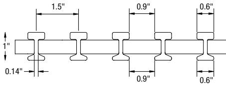
1" Deep, I-6010
