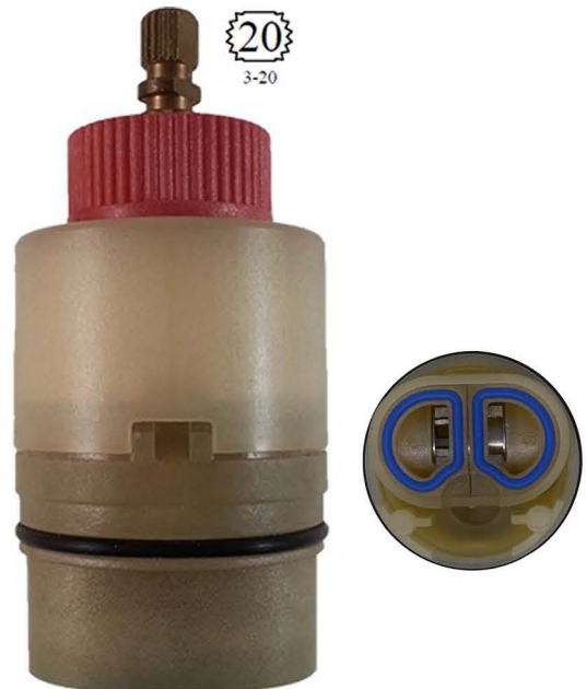
DIAMETER: 40mm CC19033
