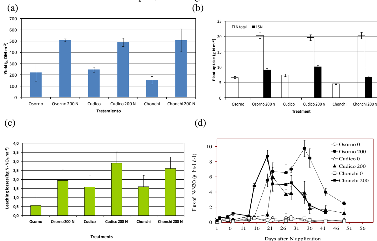
Figure 1. Nitrogen fate in volcanic ash soils with different soil organic matter content (a) yield ( \text{g DM m}^{-2} ), (b) plant uptake ( \text{g N}^{15}\text{N m}^{-2} ), (c) leaching losses ( \text{kg N-NO}_3 \text{ ha}^{-1} ), (d) flux of \text{N}_2\text{O-N} ( \text{g ha}^{-1} \text{ d}^{-1} ).
