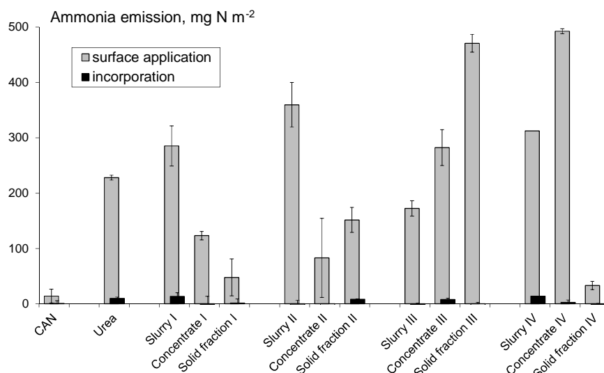
Figure 1. Total \text{NH}_3 emission (average \pm s.e.) in experiment I (arable soil). The roman numerals indicate the four different slurries, concentrates and solid fractions).
