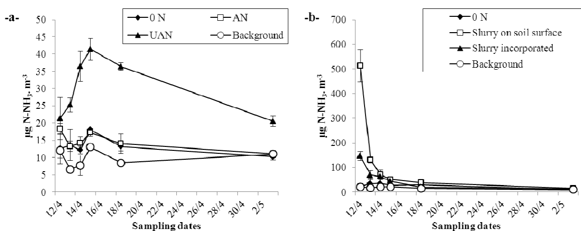
Figure 1. Ammonia concentrations at 30 cm height following mineral fertilizer applications in Bernienville 2011 experiment (-a-) and cattle slurry application in Derval 2011 experiment (-b-). Vertical bars are standard deviations.
