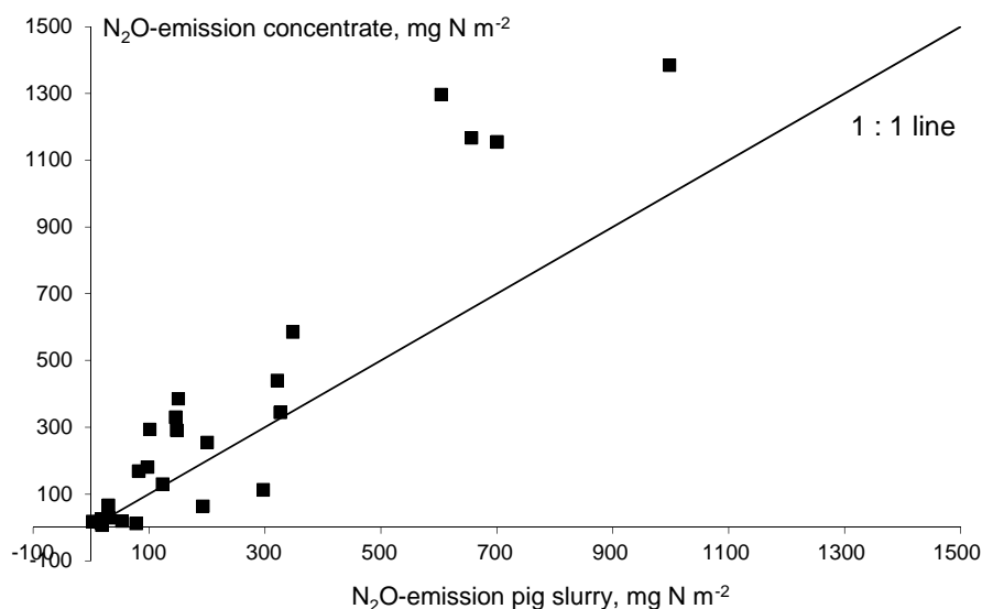
Figure 2. \text{N}_2\text{O} emission from pig slurry against \text{N}_2\text{O} emission from mineral concentrate. Results of all experiments.
