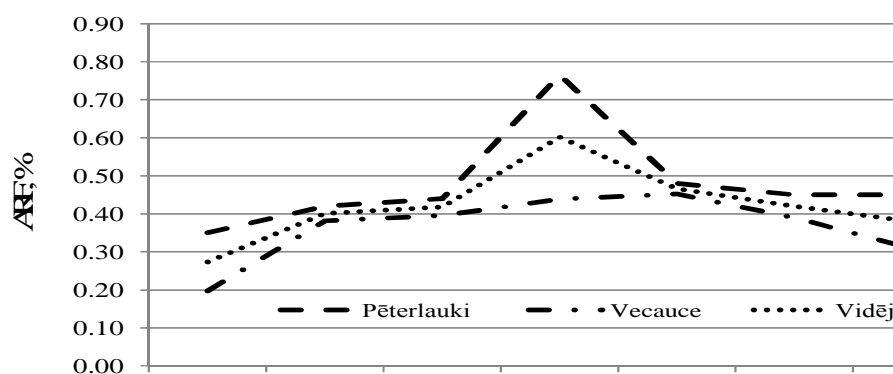
Figure 2. Average apparent recovery fraction for nitrogen depending on N rates and location of trial sites.
