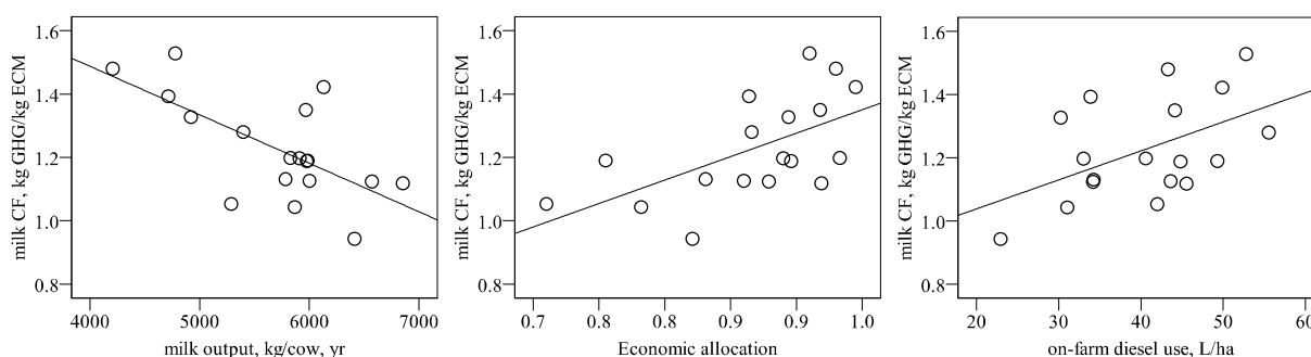
Figure 1. Relationship between milk CF and Left: milk output per cow ( r^2 = 0.43 , p < 0.001 ), middle: economic allocation factor ( r^2 = 0.36 , p < 0.001 ); right: on-farm diesel use ( r^2 = 0.25 , p < 0.05 ).
