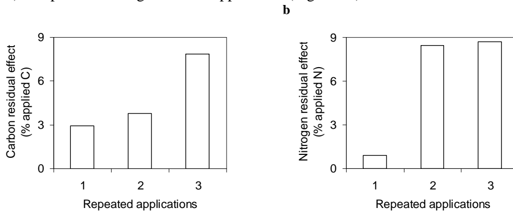
Figure 1. Carbon (a) and nitrogen (b) residual effects of a liquid dairy cow manure applied to a clay-loam soil.
