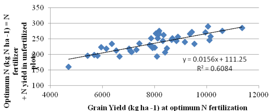
Figure 2. Winter wheat N demand (kg N ha -1 ) at optimum N rate in relation to grain yield at the optimum N rate from 44 trials in central Sweden from year 2007 to 2011. All varieties except Harnesk and Hereford.
