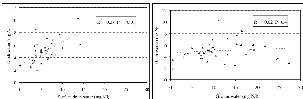
Figure 1: Correlation between total nitrogen in surface drain water and ditchwater (a) and groundwater and ditch water (b) for 8 farms in 5 year, total 40 observations.
