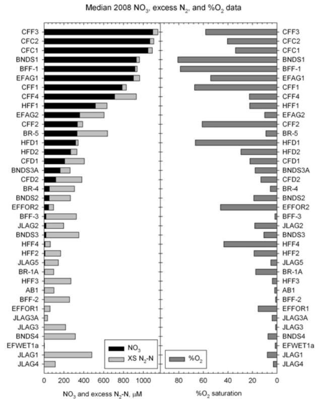
Figure 1. Spatial variations in median NO 3 - , excess N 2 , and O 2 in groundwater in the Choptank Basin. The Y axes are individual piezometers, the upper ¼ are in agricultural fields while the lower ¼ are in wetlands adjacent or within agricultural fields.
