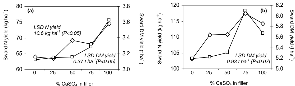
Figure 1. Effect of replacing \text{CaCO}_3 with \text{CaSO}_4 , as filler, on sward N (filled diamond) and DM (open square) yields at Terry's Hill on plots fertilised with (a) 50 kg N ha -1 at 2 nd cut 2001, and (b) with 75 kg N ha -1 at 1 st cut 2002.
