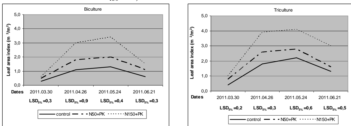
Figure 1. Dynamics of LAI-values of winter wheat in a bi- and triculture crop-rotation system (Debrecen, 2011.)
