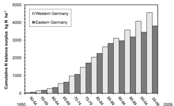
Figure 2: Cumulative N surpluses in Germany (Adapted from Nieder et al., 2007)
