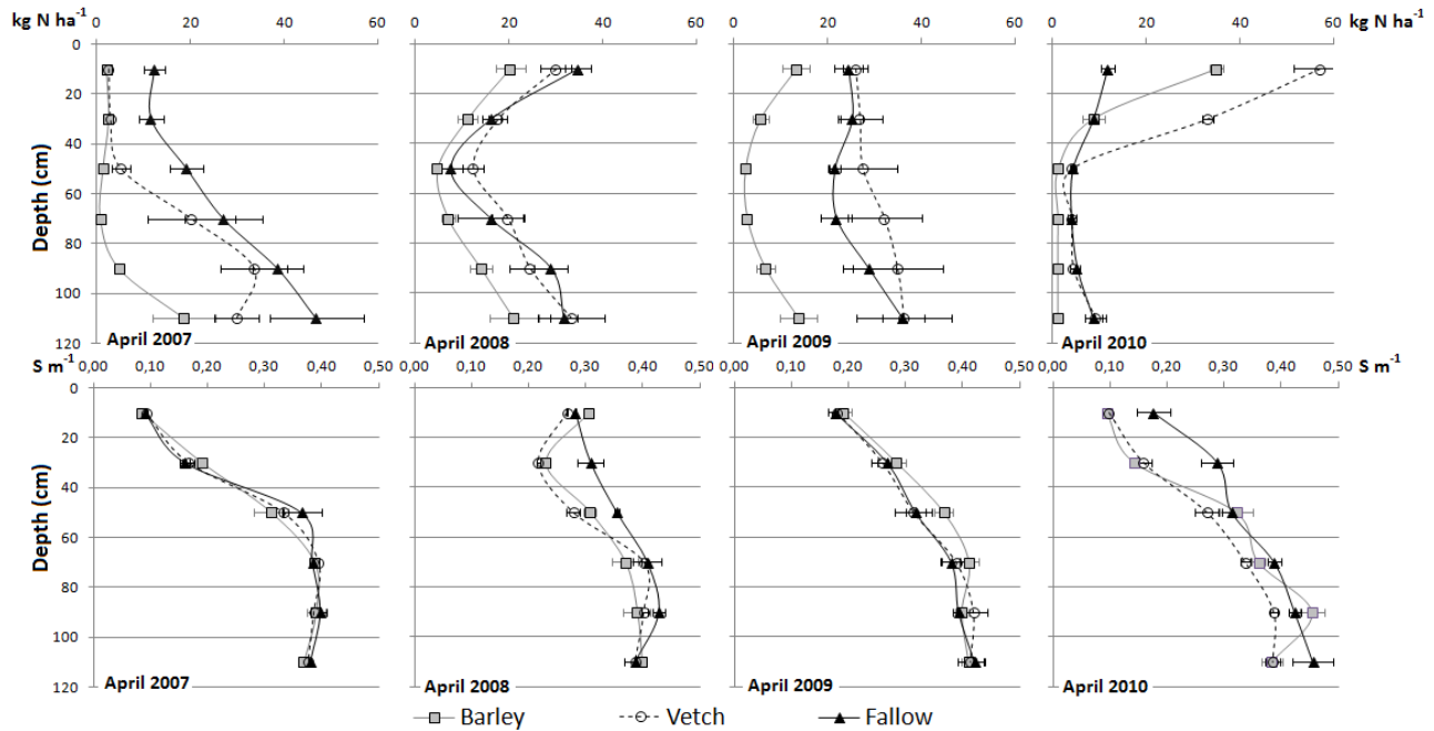
Figure 2. Distribution of soil \text{N}_{\text{min}} ( \text{kg N ha}^{-1} ) and saturated paste extract soil electrical conductivity ( \text{S m}^{-1} ) by depth at the end of the cover crop growing season (maize sowing), as influenced by the cover crop treatment.
