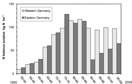
Figure 1: N surpluses in Germany 1950-2009 (Adapted from Nieder et al., 2007)
